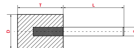
MOUNTED POINTS
